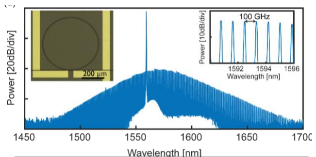
Figure. Spectrum of an integrated frequency comb. The left inset shows the microfabricated device with thermo-optic heaters on top. The right inset is a zoom in of the spectrum, showing the comb teeth, spaced in frequency by 100 GHz.
